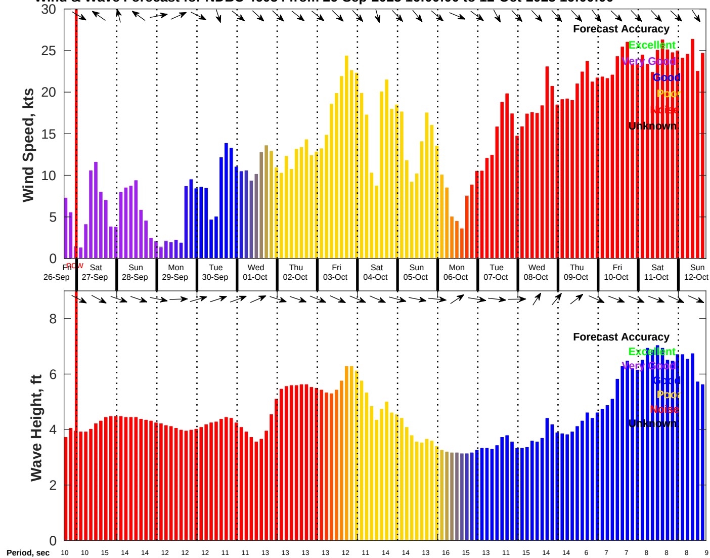
Wind & Wave Forecast for NDBC 46054 from 26-Sep-2025 16:00:00 to 12-Oct-2025 16:00:00
