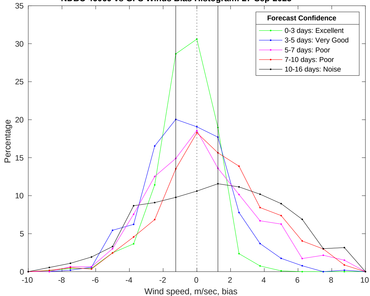
NDBC 46069 vs GFS Winds Bias Histogram: 27-Sep-2025
