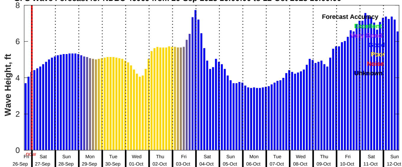
GFS Wave Forecast for NDBC 46069 from 26-Sep-2025 16:00:00 to 12-Oct-2025 16:00:00
