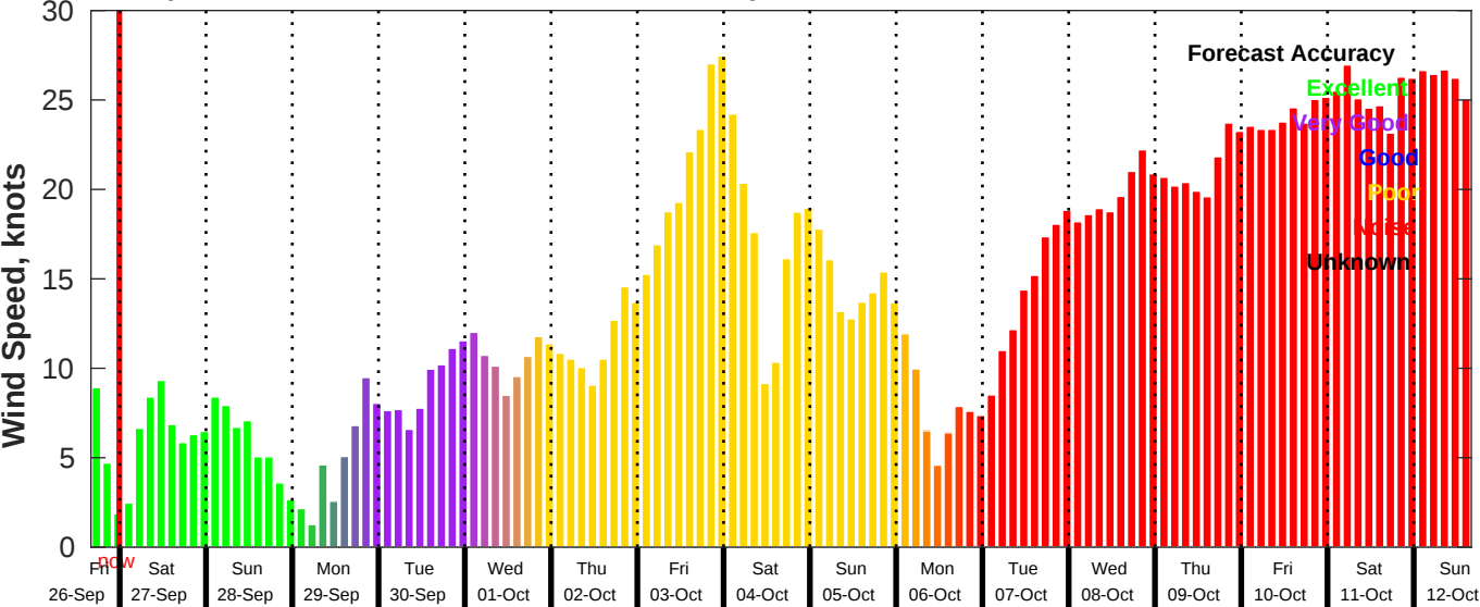
GFS Wind Speed Forecast for NDBC 46069 from 26-Sep-2025 16:00:00 to 12-Oct-2025 16:00:00
