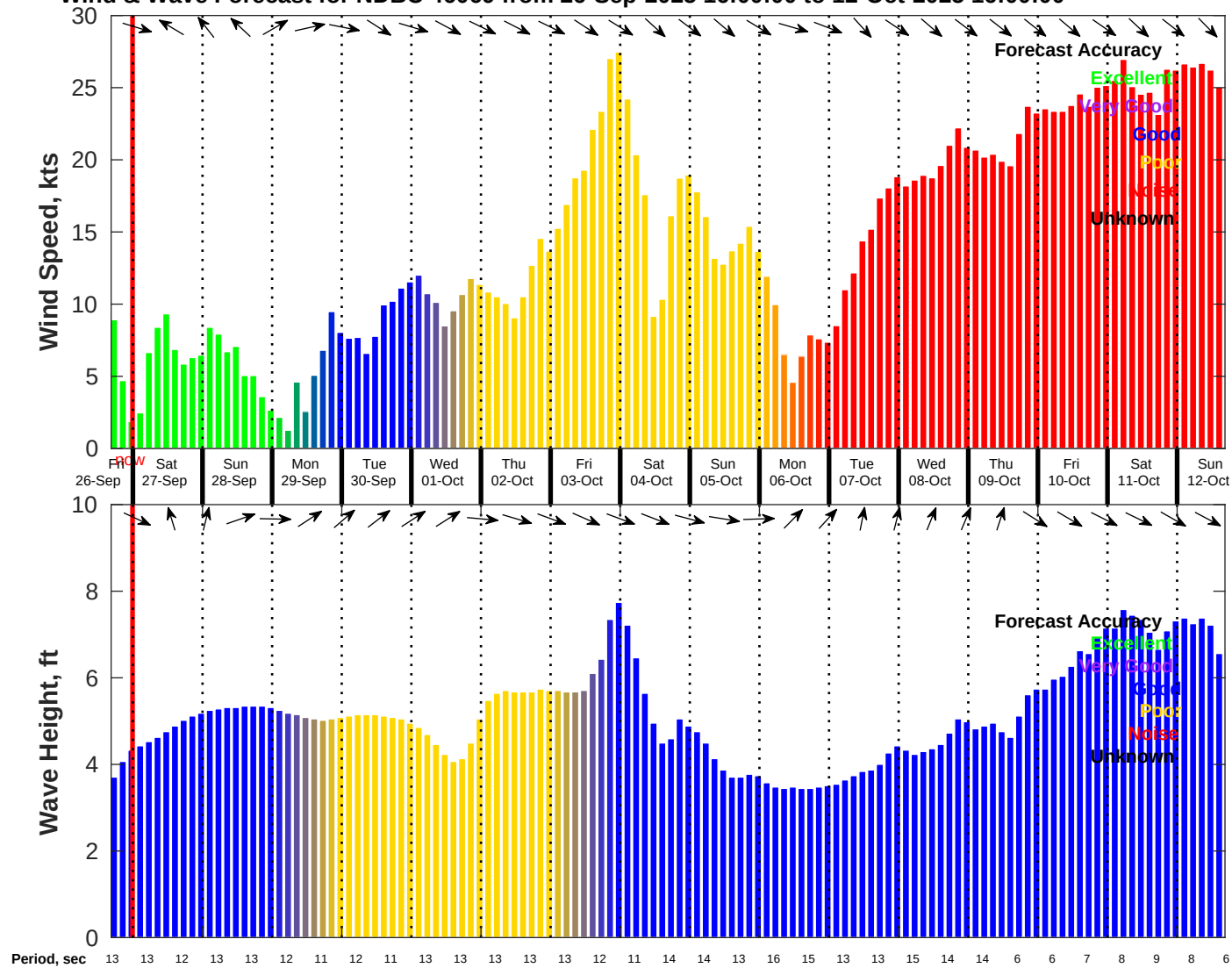
Wind & Wave Forecast for NDBC 46069 from 26-Sep-2025 16:00:00 to 12-Oct-2025 16:00:00
