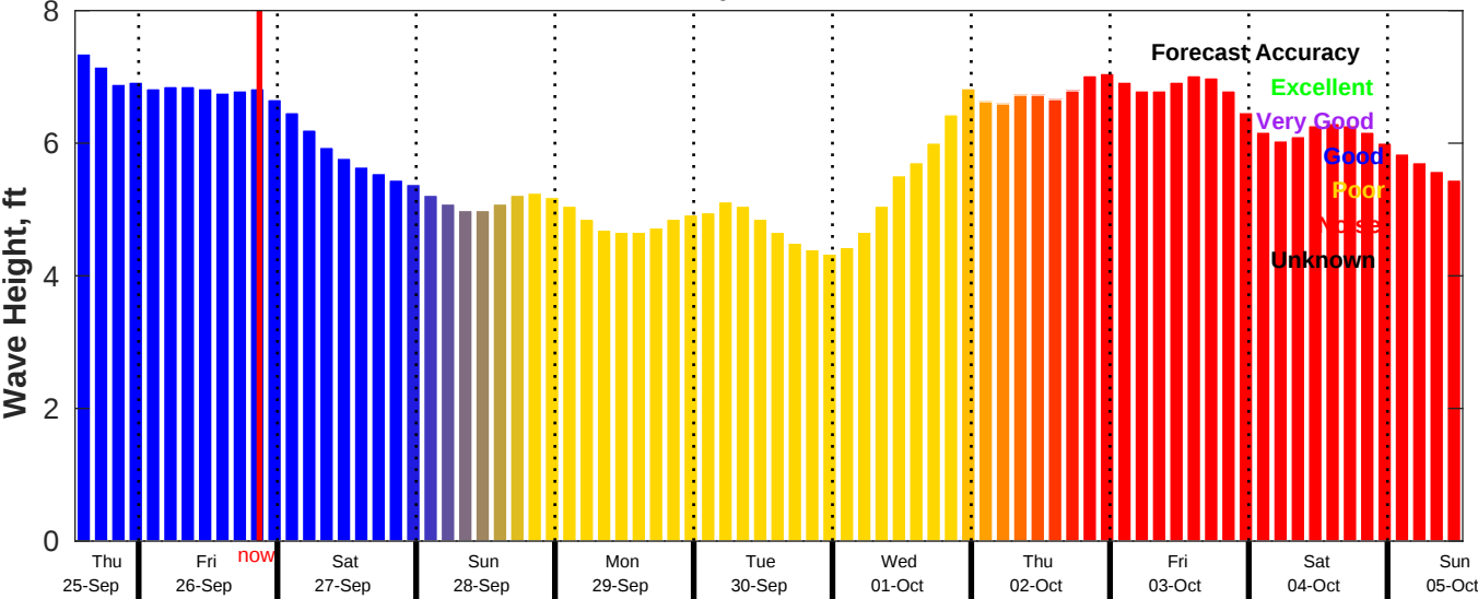
CMEMS Wave Forecast for NDBC 51209 from 25-Sep-2025 13:00:00 to 05-Oct-2025 13:00:00
