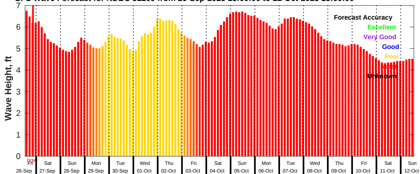
GFS Wave Forecast for NDBC 51209 from 26-Sep-2025 13:00:00 to 12-Oct-2025 13:00:00
