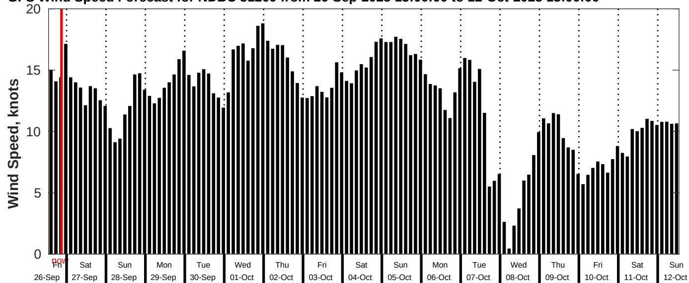
GFS Wind Speed Forecast for NDBC 51209 from 26-Sep-2025 13:00:00 to 12-Oct-2025 13:00:00
