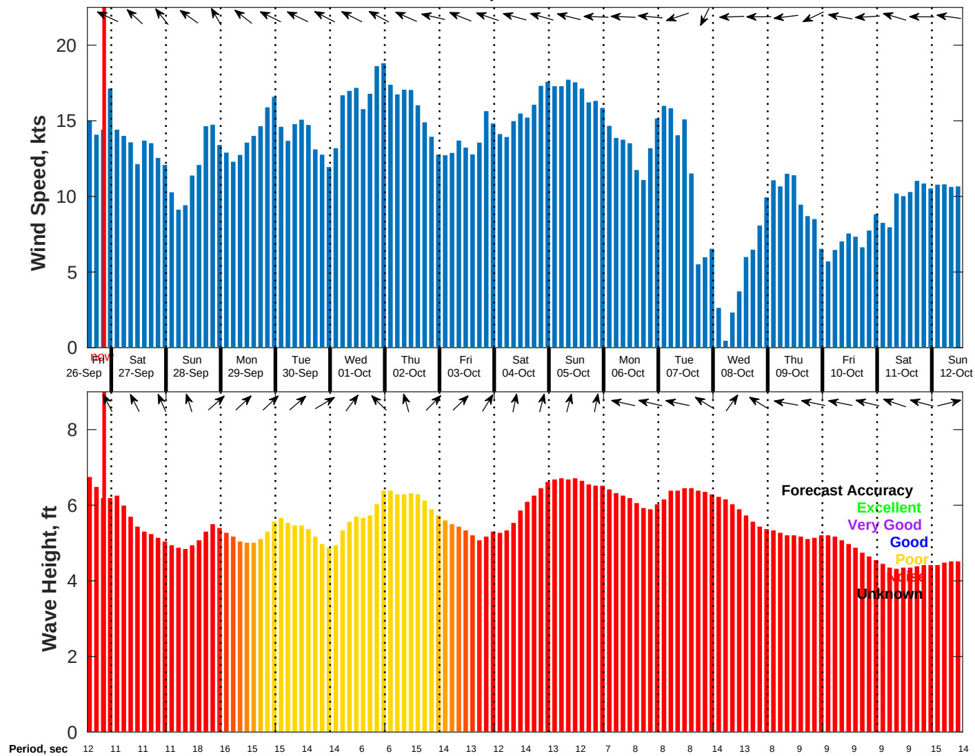
Wind & Wave Forecast for NDBC 51209 from 26-Sep-2025 13:00:00 to 12-Oct-2025 13:00:00
