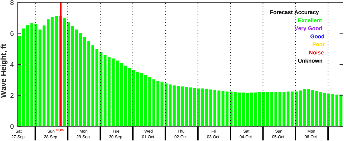
CMEMS Wave Forecast for NDBC 52211 from 26-Sep-2025 11:00:00 to 06-Oct-2025 11:00:00
