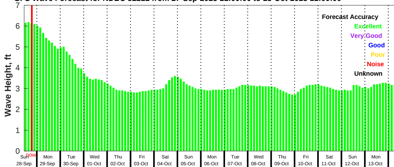
GFS Wave Forecast for NDBC 52211 from 27-Sep-2025 11:00:00 to 13-Oct-2025 11:00:00
