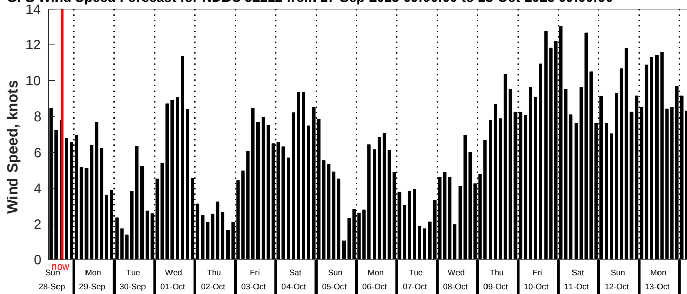
GFS Wind Speed Forecast for NDBC 52212 from 27-Sep-2025 09:00:00 to 13-Oct-2025 09:00:00
