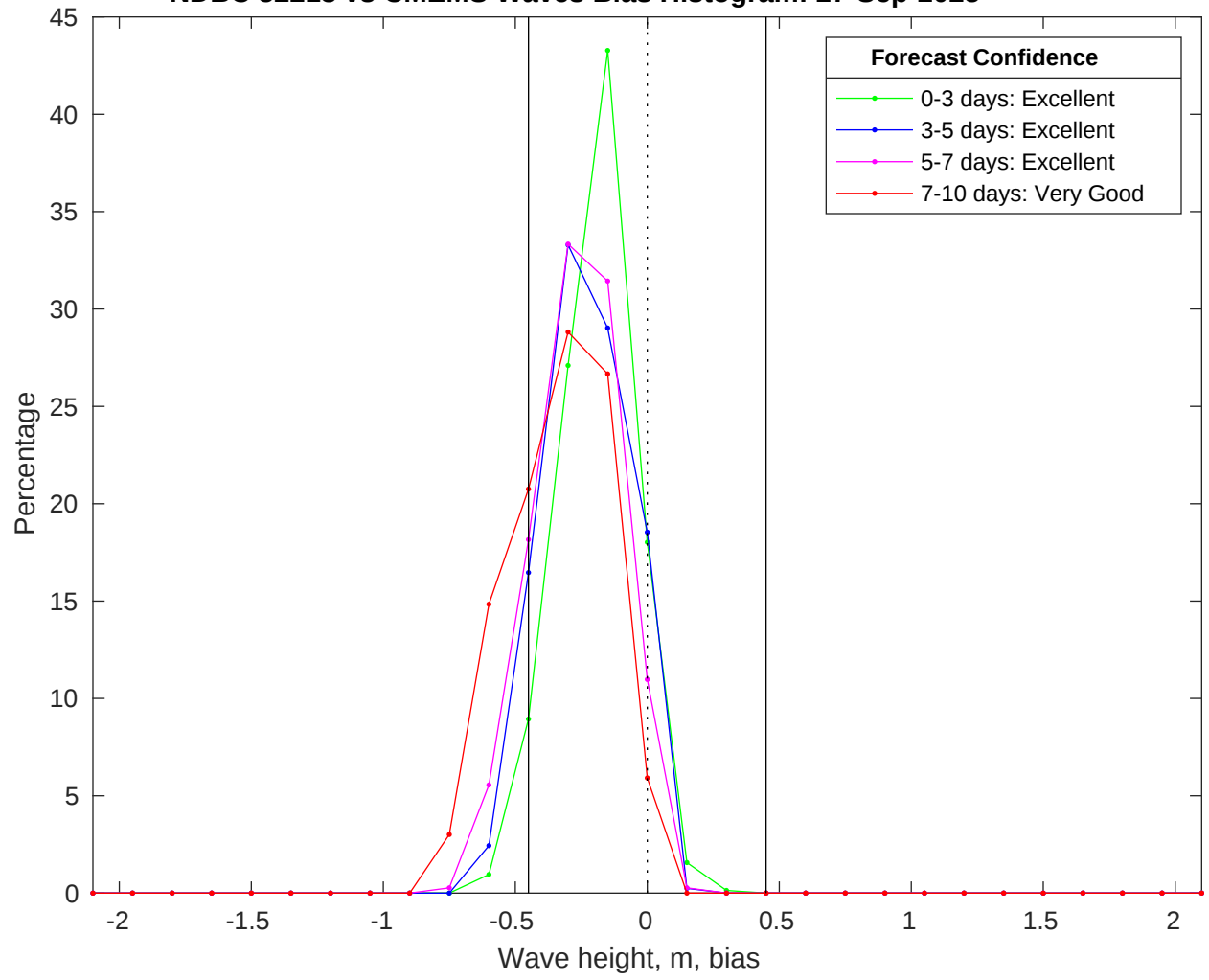
NDBC 52213 vs CMEMS Waves Bias Histogram: 27-Sep-2025
