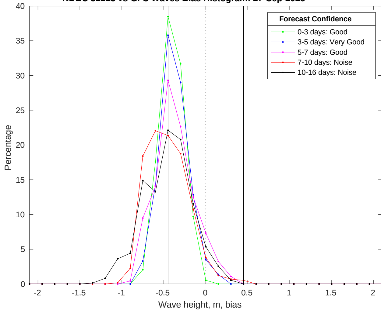
NDBC 52213 vs GFS Waves Bias Histogram: 27-Sep-2025
