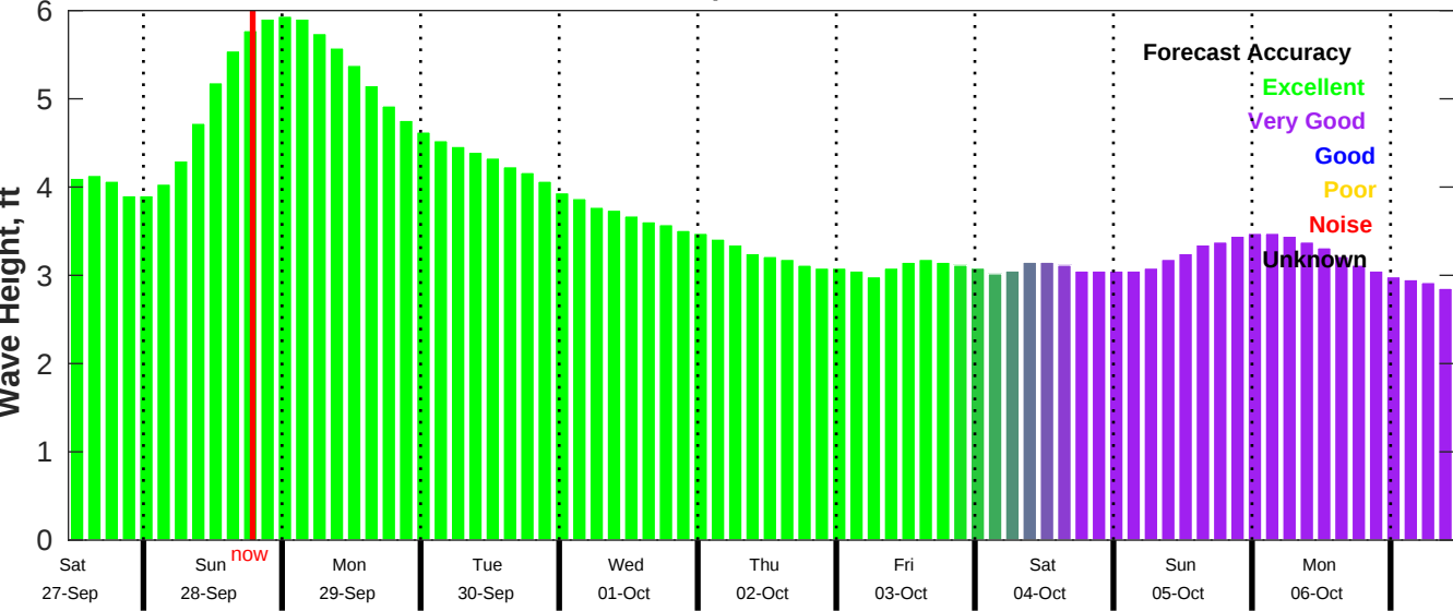
CMEMS Wave Forecast for NDBC 52213 from 26-Sep-2025 11:00:00 to 06-Oct-2025 11:00:00
