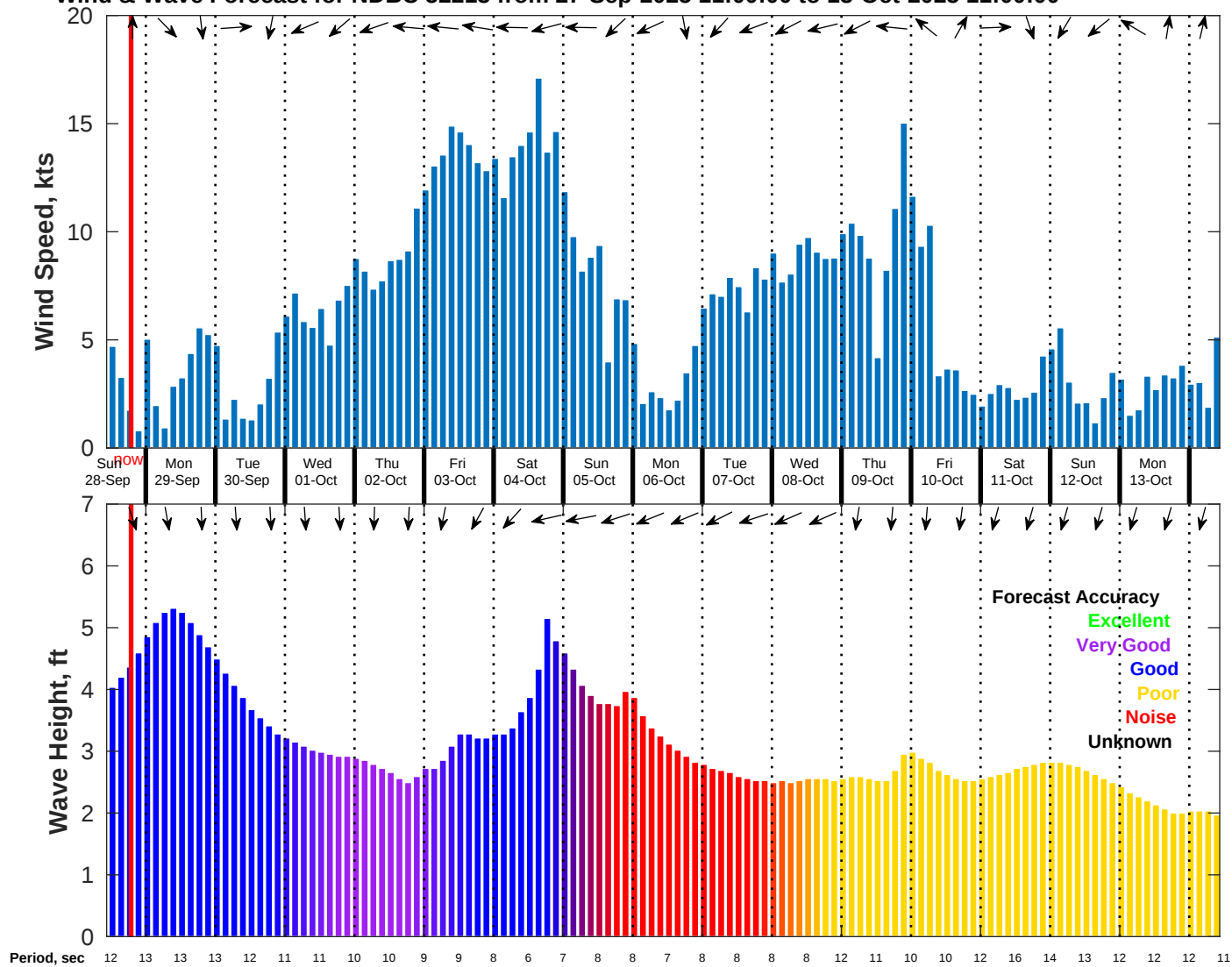
Wind & Wave Forecast for NDBC 52213 from 27-Sep-2025 11:00:00 to 13-Oct-2025 11:00:00
