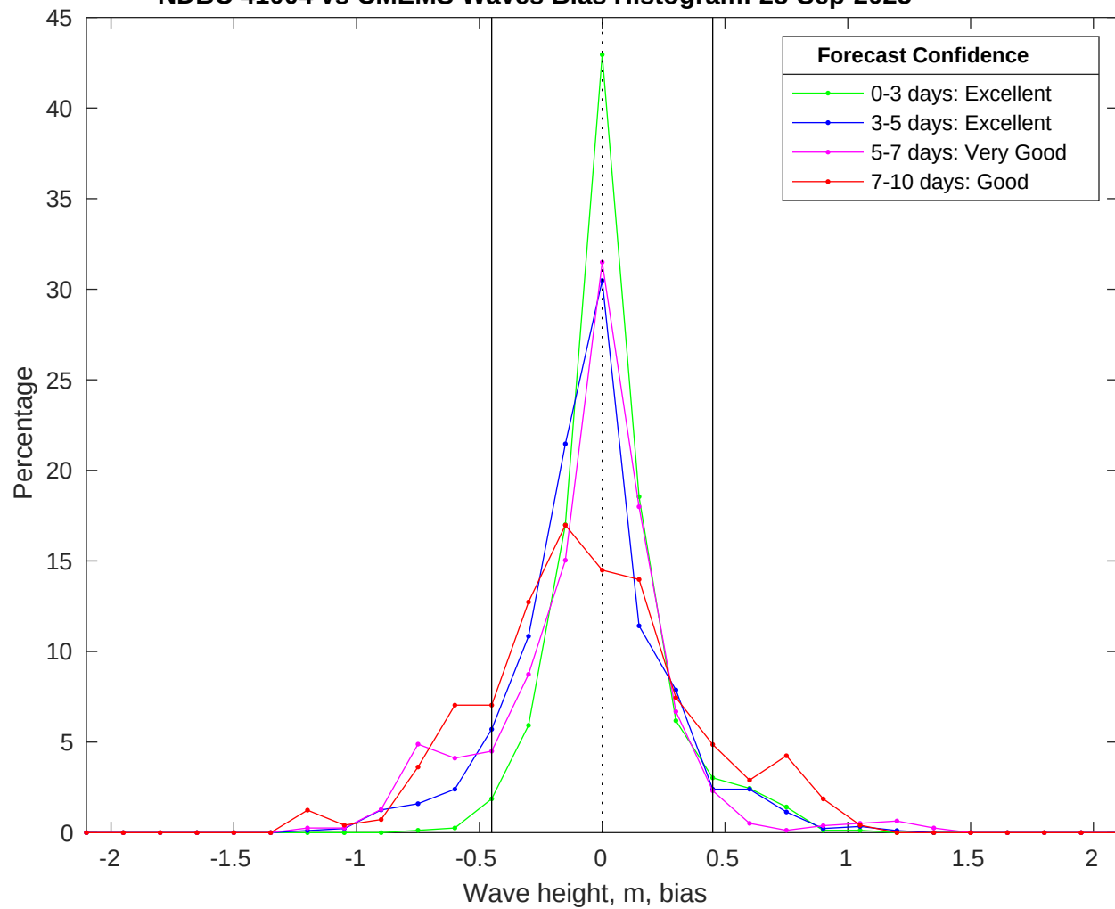
NDBC 41004 vs CMEMS Waves Bias Histogram: 28-Sep-2025
