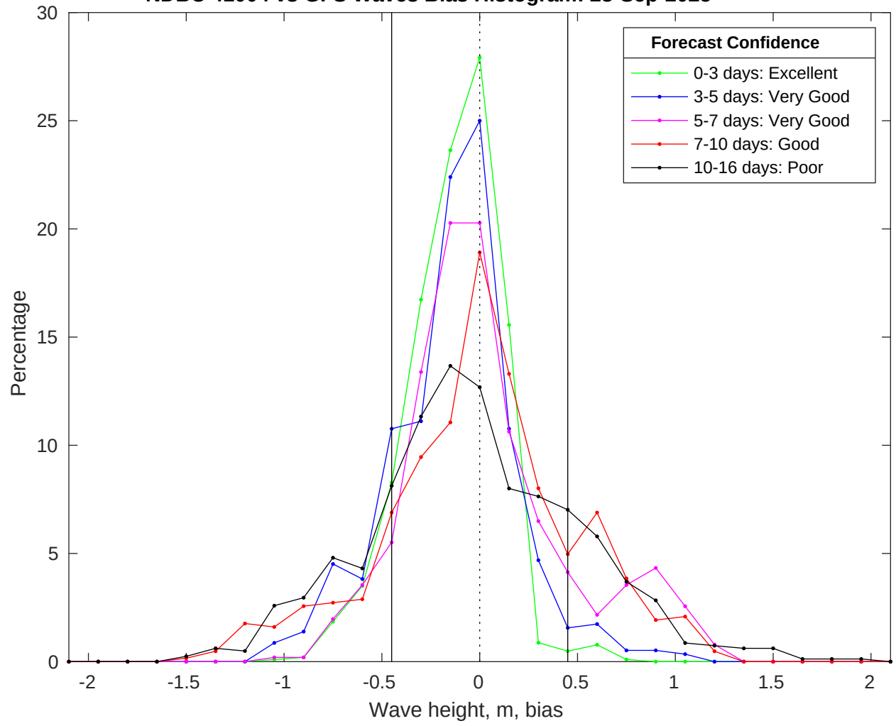
NDBC 41004 vs GFS Waves Bias Histogram: 28-Sep-2025
