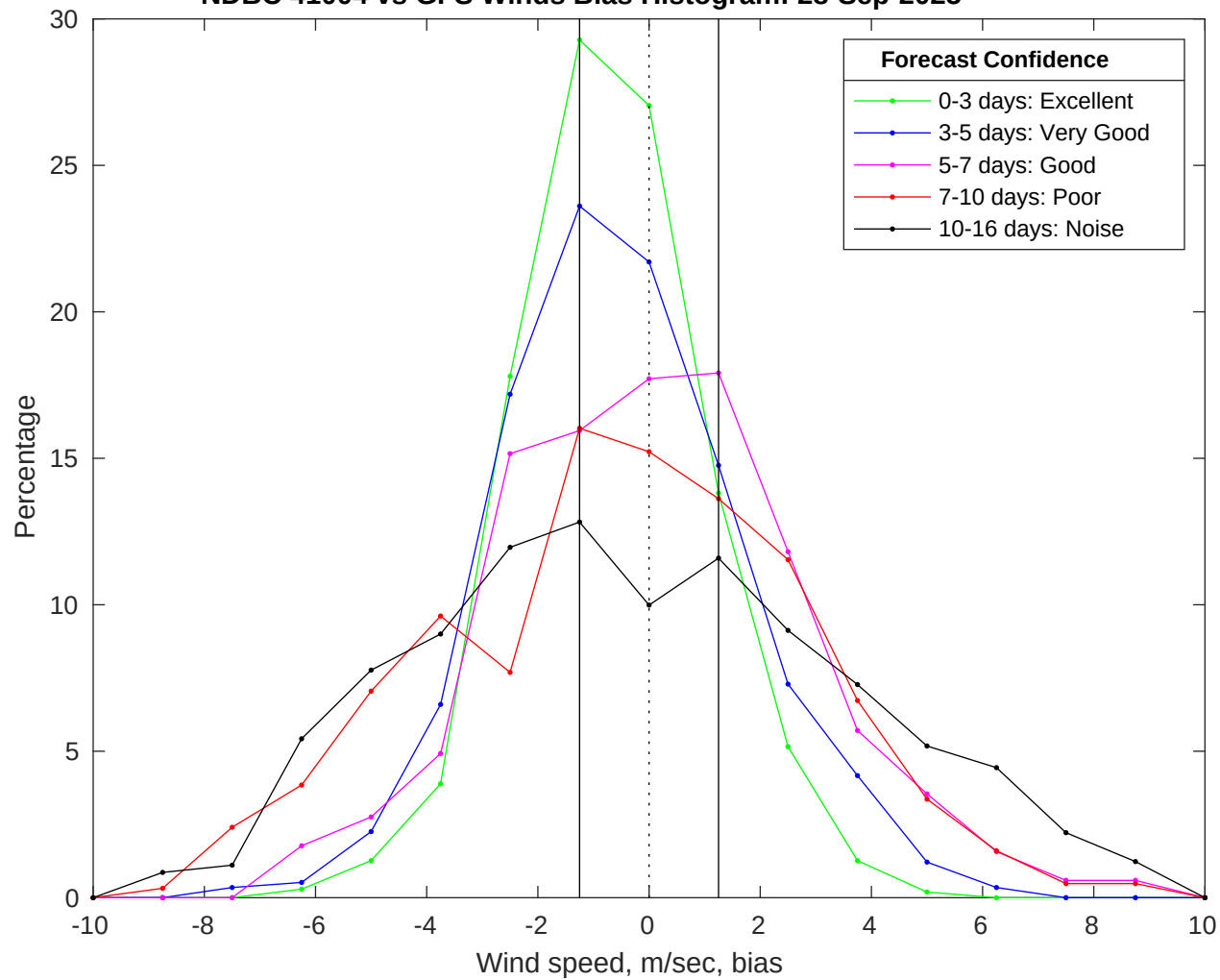
NDBC 41004 vs GFS Winds Bias Histogram: 28-Sep-2025
