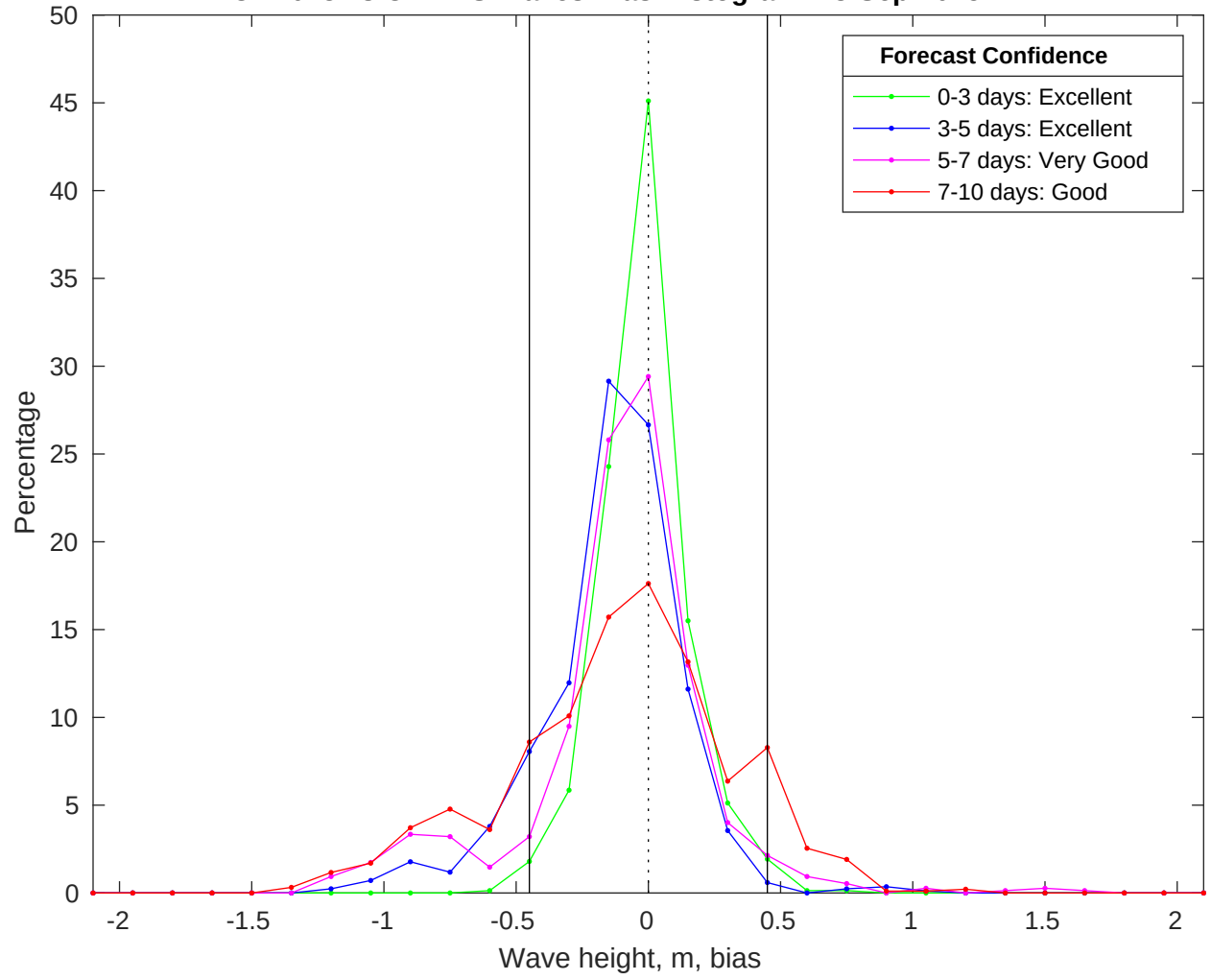
NDBC 41013 vs CMEMS Waves Bias Histogram: 28-Sep-2025
