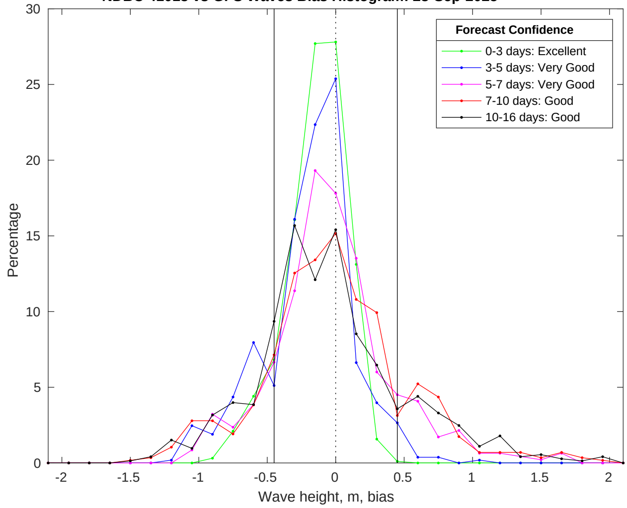
NDBC 41013 vs GFS Waves Bias Histogram: 28-Sep-2025
