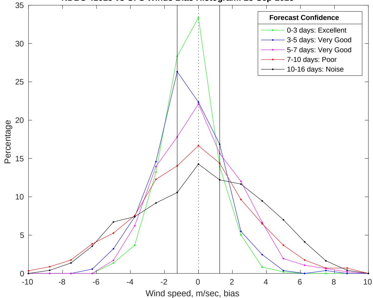
NDBC 41013 vs GFS Winds Bias Histogram: 28-Sep-2025
