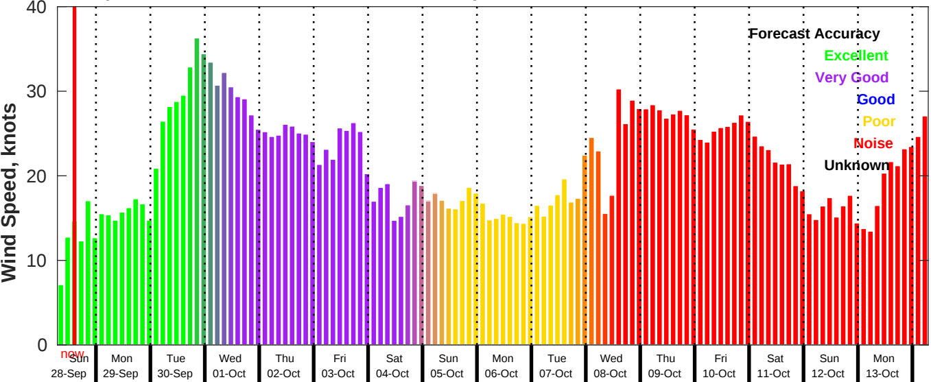
GFS Wind Speed Forecast for NDBC 41013 from 28-Sep-2025 07:00:00 to 14-Oct-2025 07:00:00
