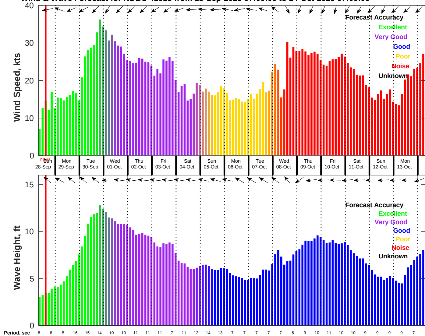
Wind & Wave Forecast for NDBC 41013 from 28-Sep-2025 07:00:00 to 14-Oct-2025 07:00:00
