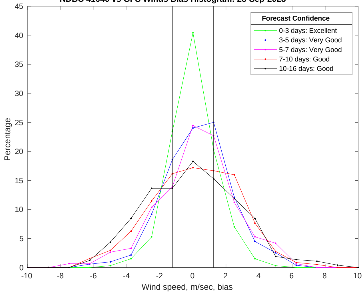
NDBC 41040 vs GFS Winds Bias Histogram: 28-Sep-2025
