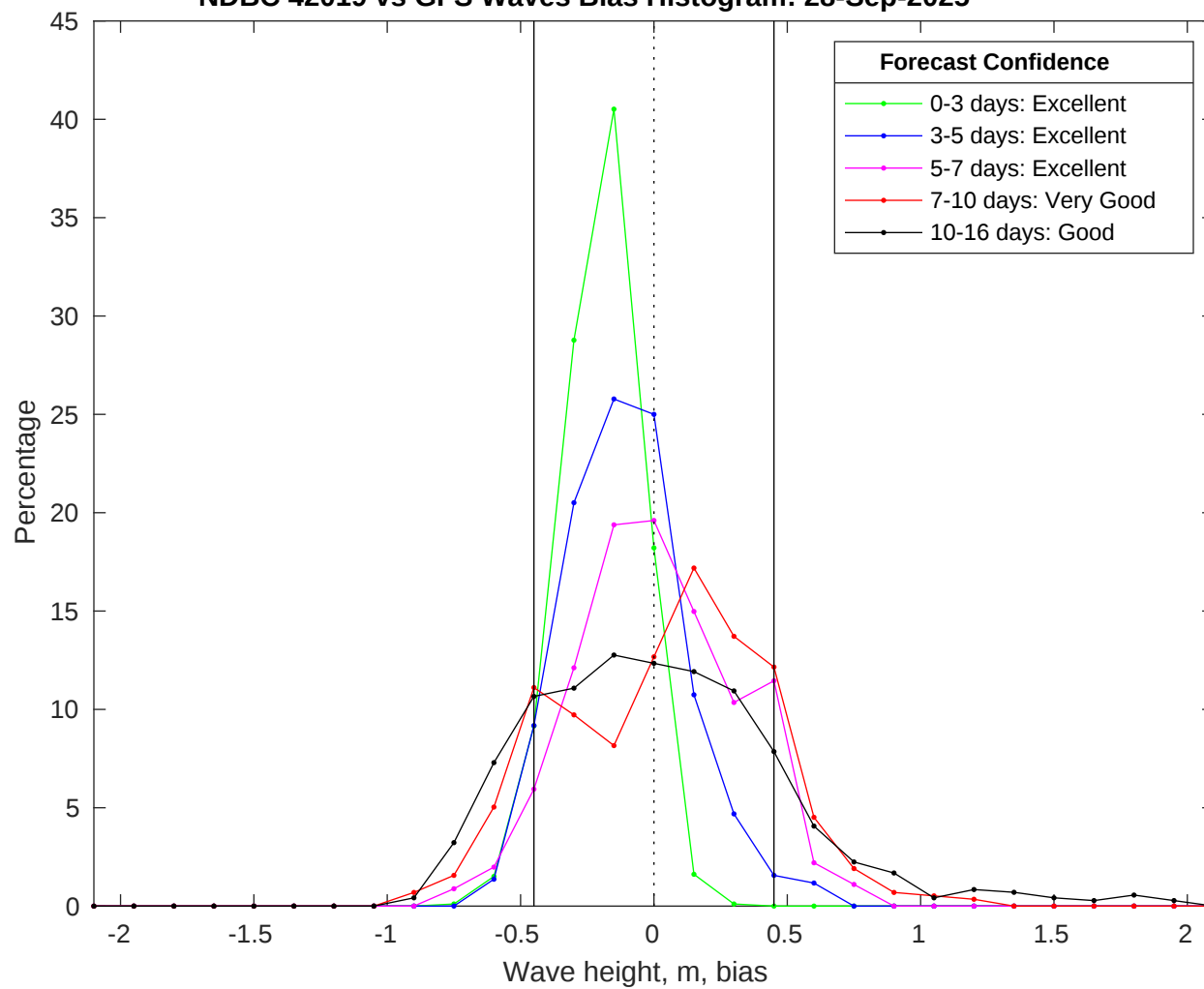
NDBC 42019 vs GFS Waves Bias Histogram: 28-Sep-2025
