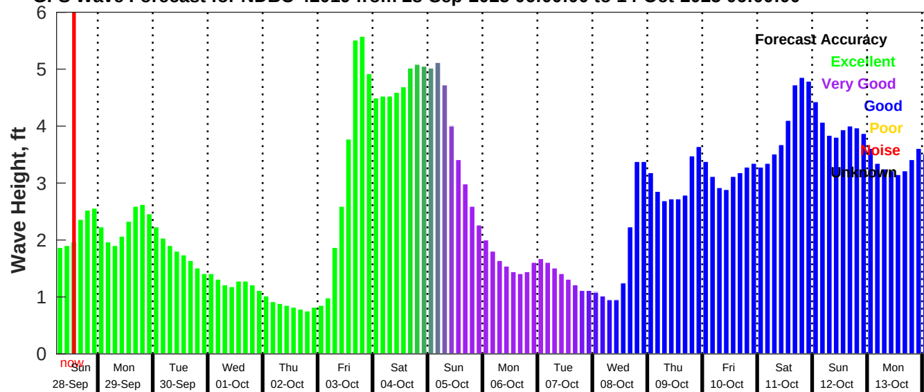
GFS Wave Forecast for NDBC 42019 from 28-Sep-2025 06:00:00 to 14-Oct-2025 06:00:00
