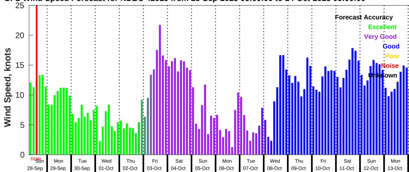
GFS Wind Speed Forecast for NDBC 42019 from 28-Sep-2025 06:00:00 to 14-Oct-2025 06:00:00
