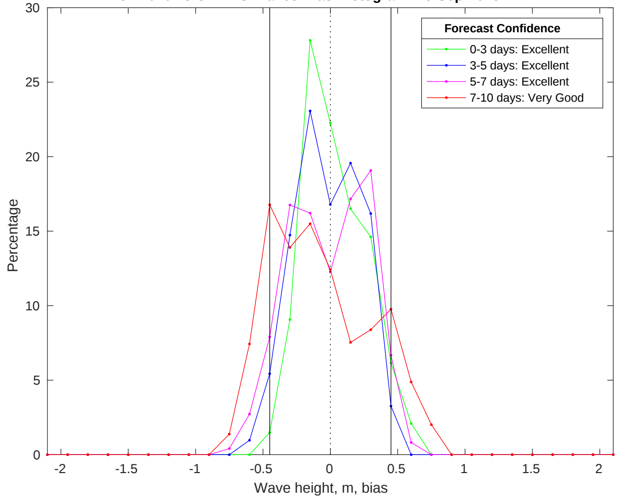
NDBC 42020 vs CMEMS Waves Bias Histogram: 28-Sep-2025
