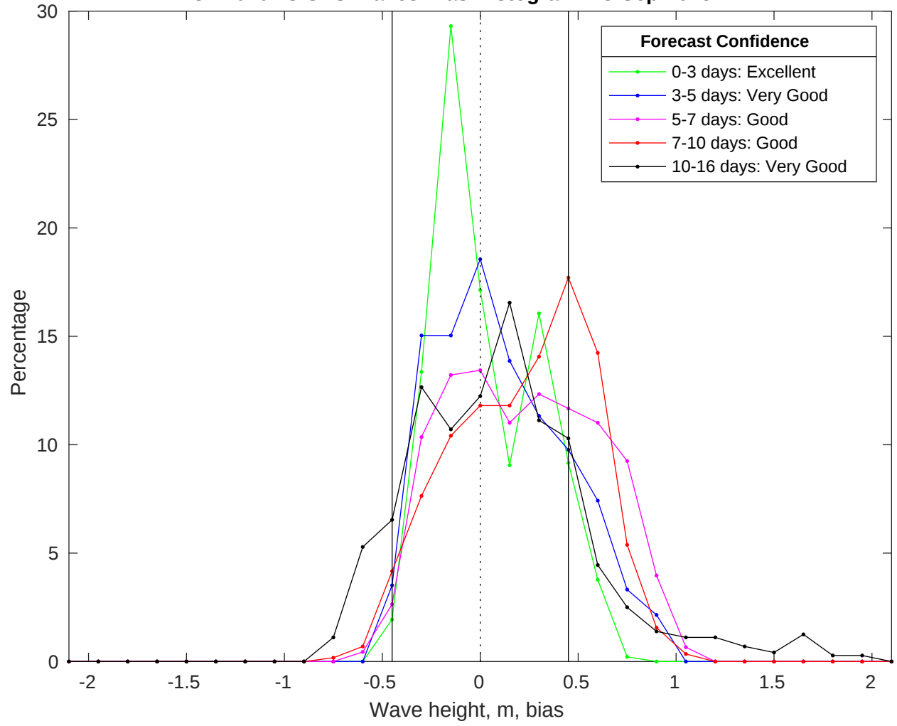
NDBC 42020 vs GFS Waves Bias Histogram: 28-Sep-2025
