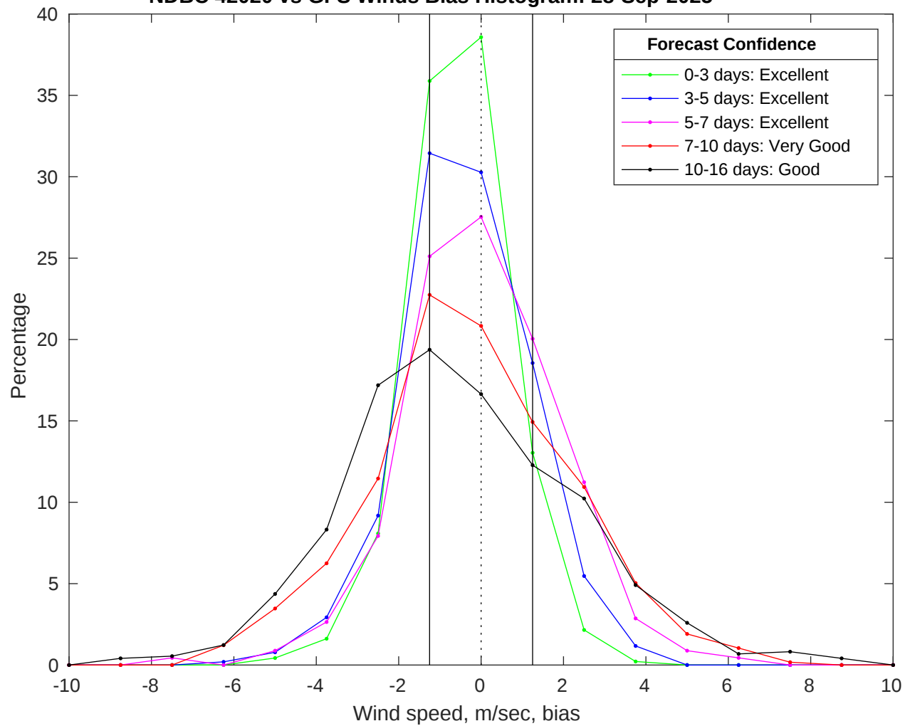
NDBC 42020 vs GFS Winds Bias Histogram: 28-Sep-2025
