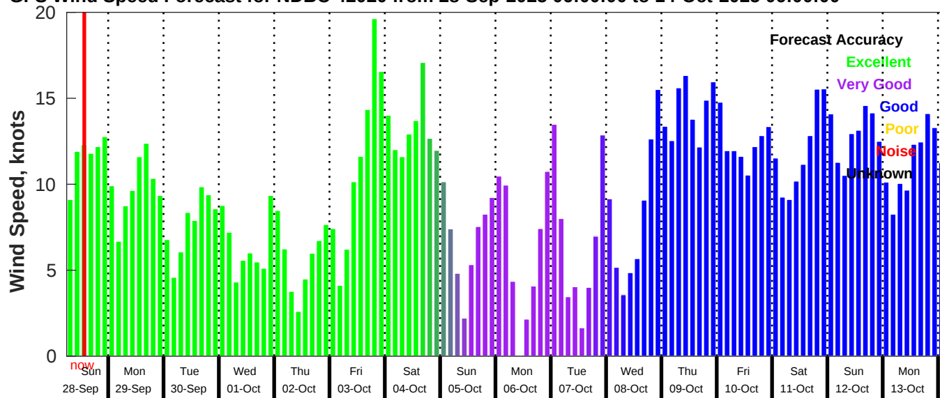
GFS Wind Speed Forecast for NDBC 42020 from 28-Sep-2025 06:00:00 to 14-Oct-2025 06:00:00
