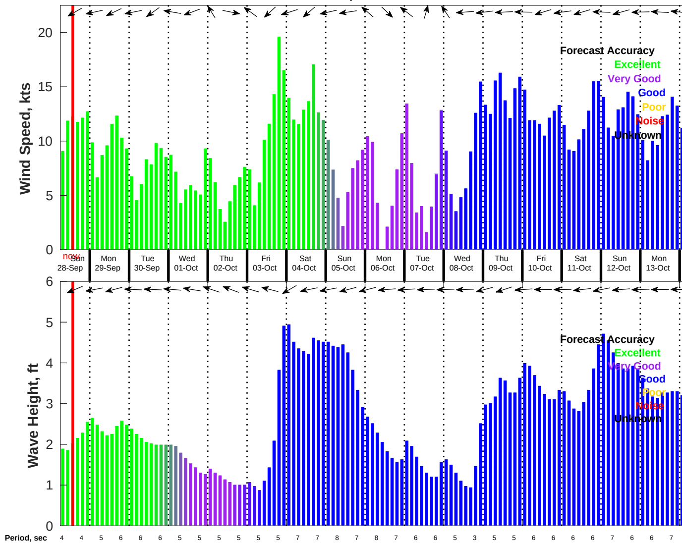
Wind & Wave Forecast for NDBC 42020 from 28-Sep-2025 06:00:00 to 14-Oct-2025 06:00:00
