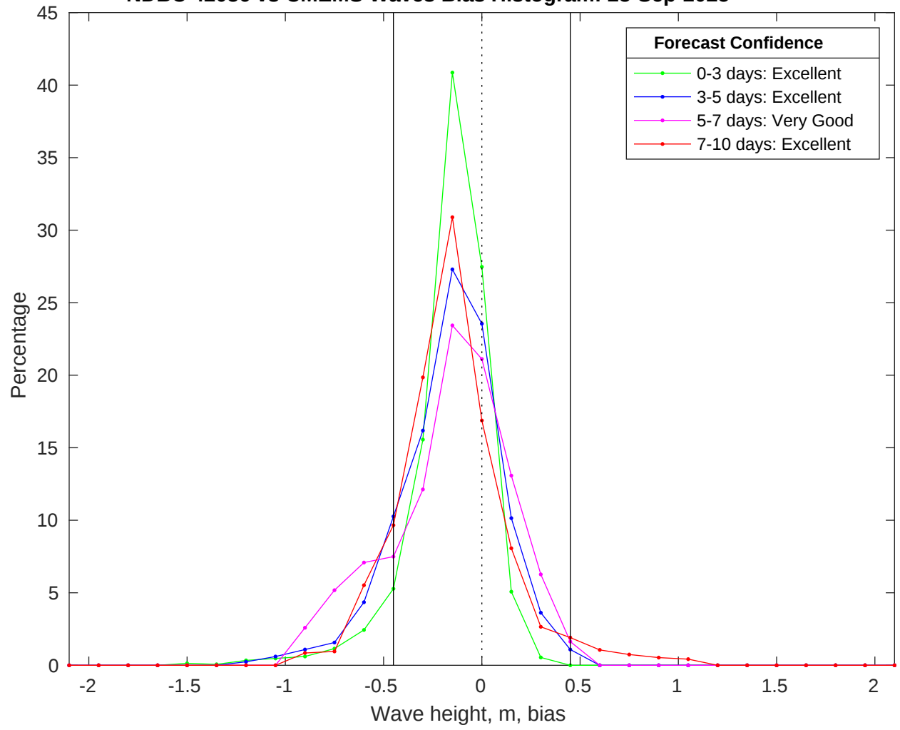
NDBC 42036 vs CMEMS Waves Bias Histogram: 28-Sep-2025
