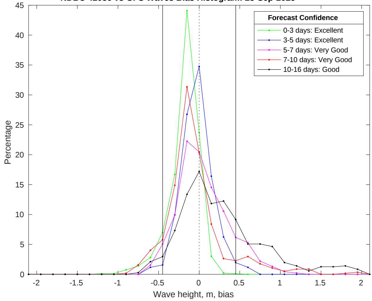
NDBC 42036 vs GFS Waves Bias Histogram: 28-Sep-2025
