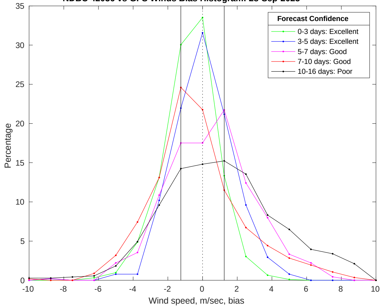
NDBC 42036 vs GFS Winds Bias Histogram: 28-Sep-2025
