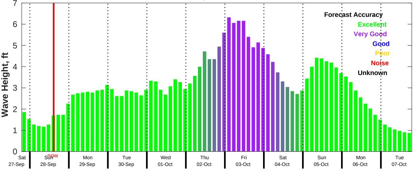
CMEMS Wave Forecast for NDBC 42036 from 27-Sep-2025 19:00:00 to 07-Oct-2025 19:00:00
