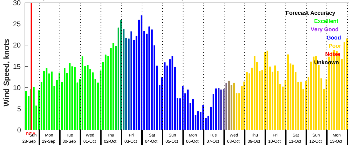
GFS Wind Speed Forecast for NDBC 42036 from 28-Sep-2025 07:00:00 to 14-Oct-2025 07:00:00
