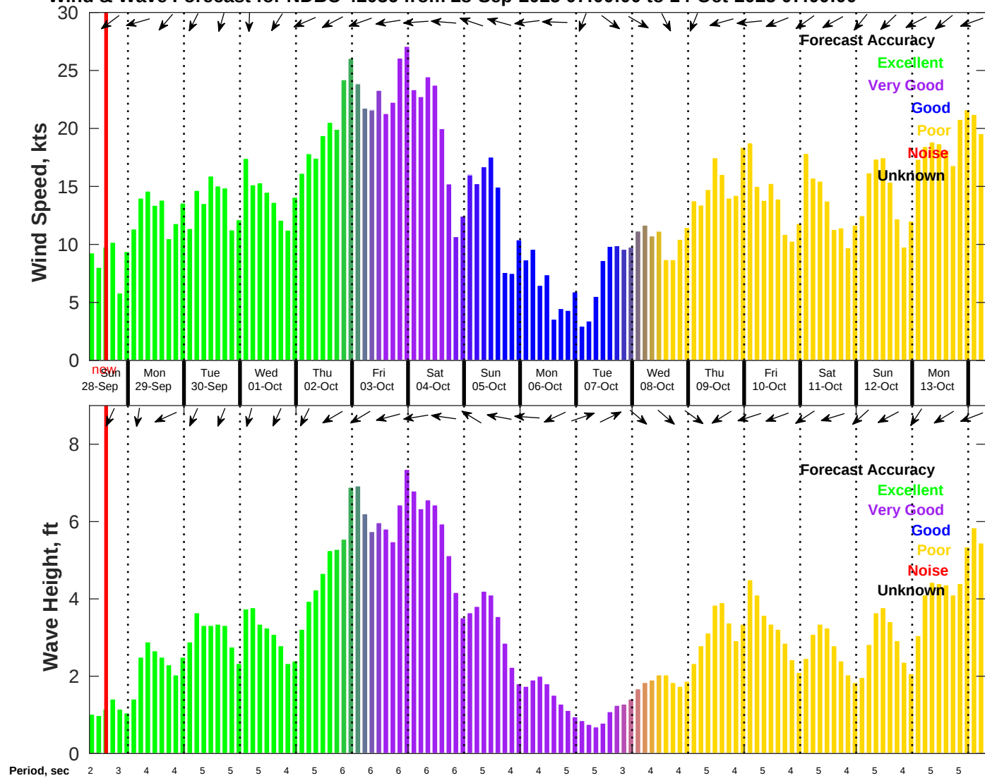
Wind & Wave Forecast for NDBC 42036 from 28-Sep-2025 07:00:00 to 14-Oct-2025 07:00:00
