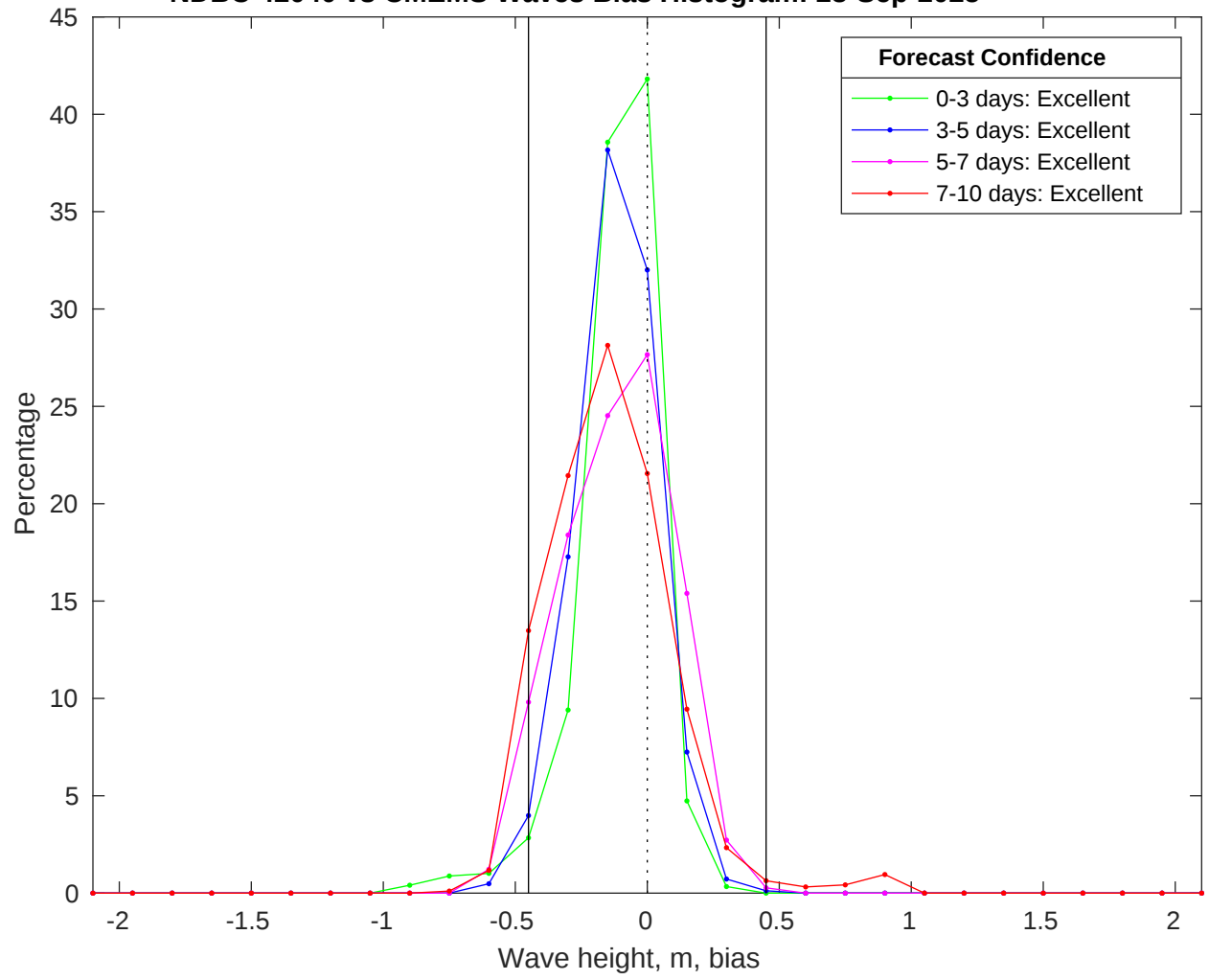
NDBC 42040 vs CMEMS Waves Bias Histogram: 28-Sep-2025
