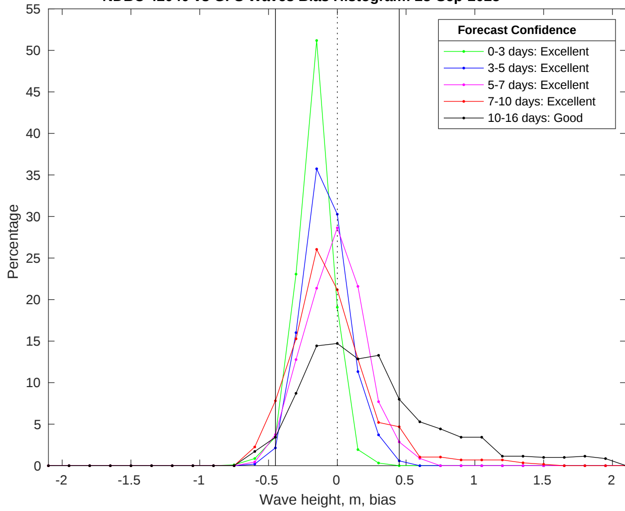
NDBC 42040 vs GFS Waves Bias Histogram: 28-Sep-2025
