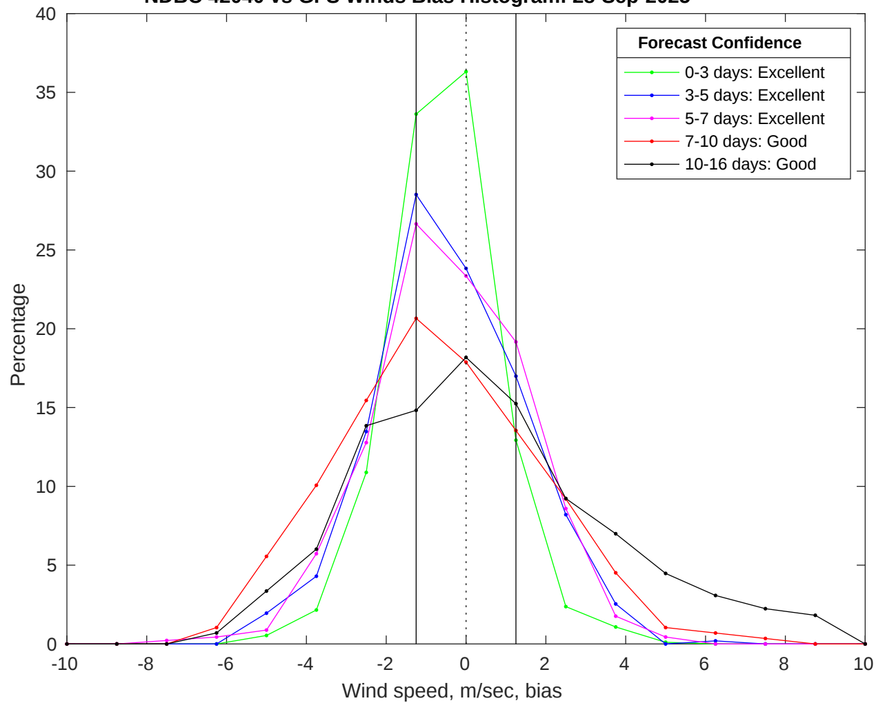
NDBC 42040 vs GFS Winds Bias Histogram: 28-Sep-2025
