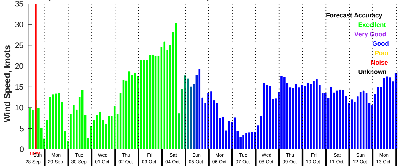
GFS Wind Speed Forecast for NDBC 42040 from 28-Sep-2025 07:00:00 to 14-Oct-2025 07:00:00
