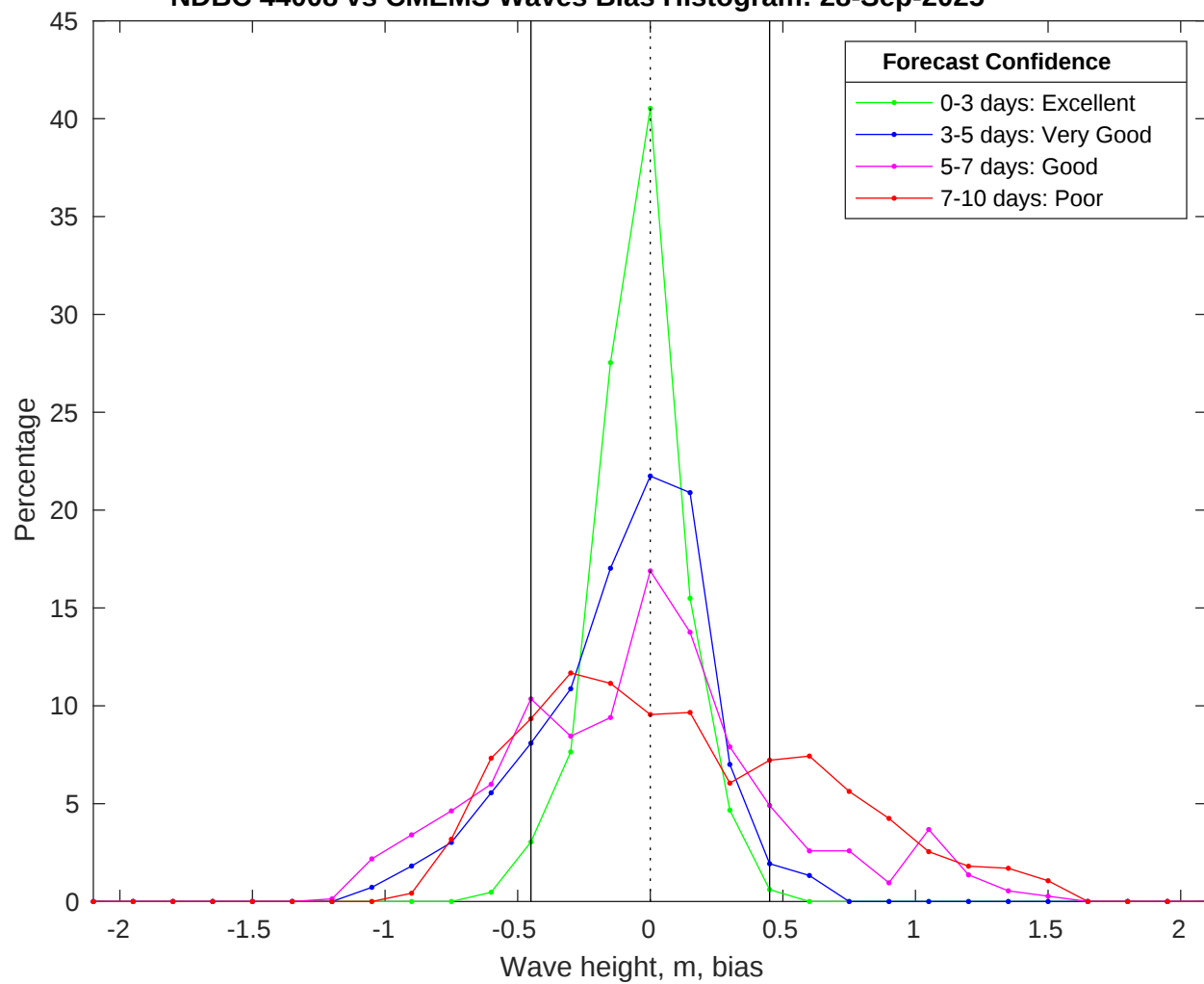
NDBC 44008 vs CMEMS Waves Bias Histogram: 28-Sep-2025
