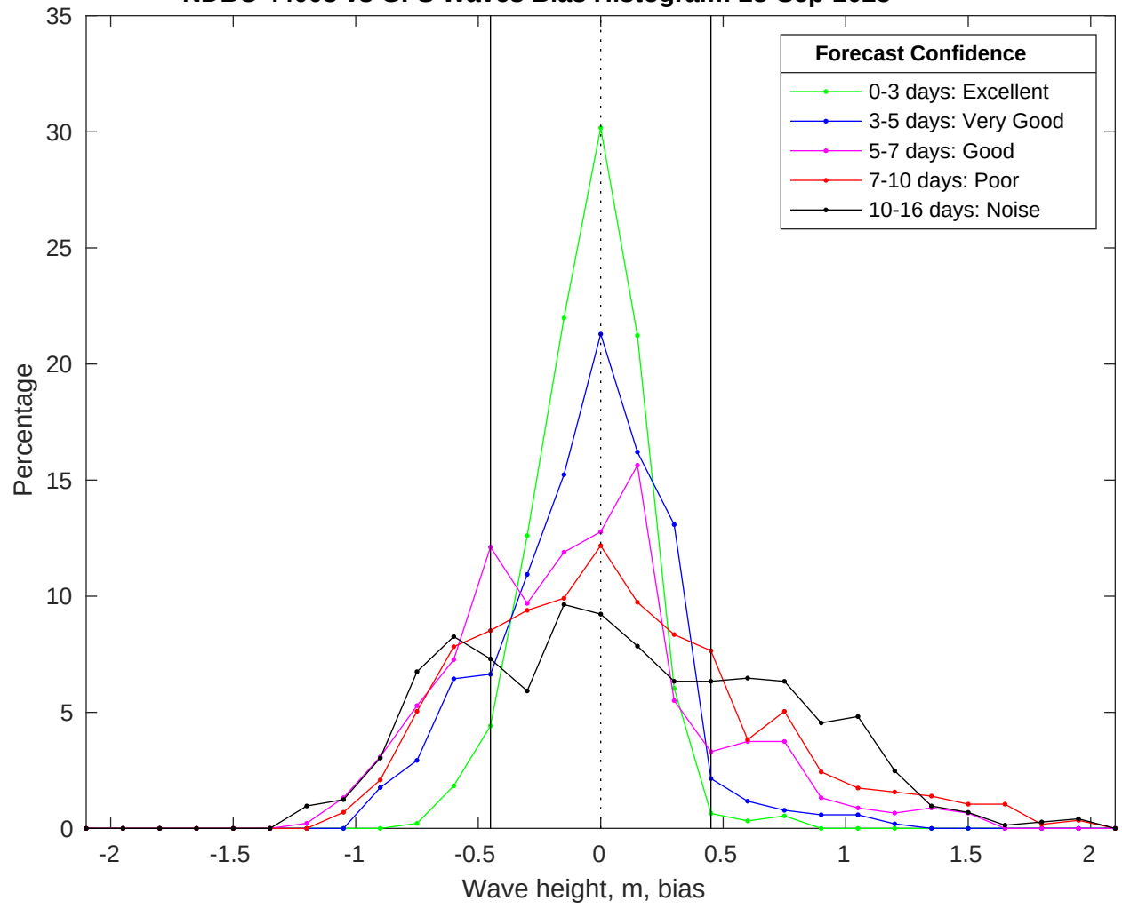
NDBC 44008 vs GFS Waves Bias Histogram: 28-Sep-2025
