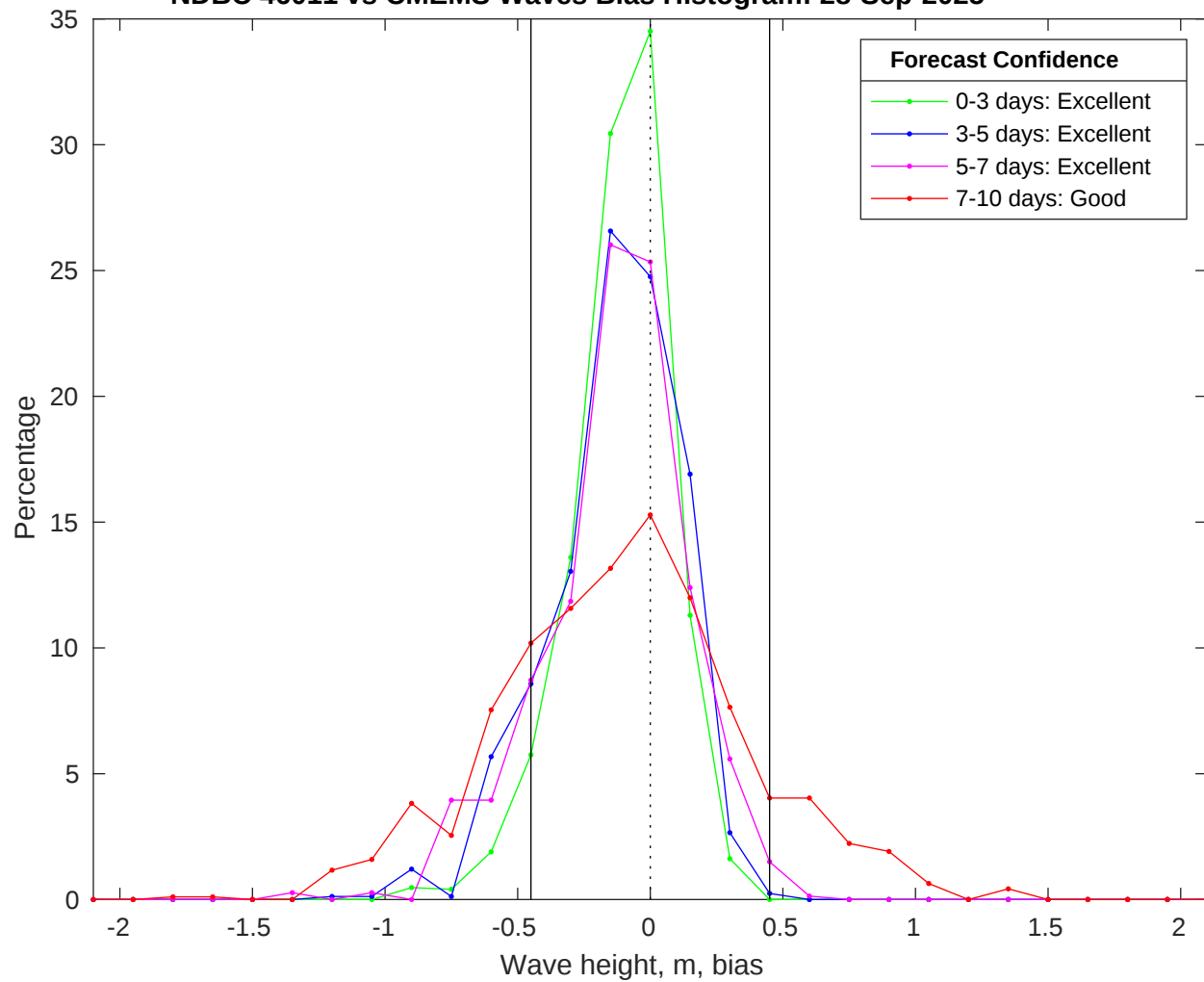
NDBC 46011 vs CMEMS Waves Bias Histogram: 28-Sep-2025
