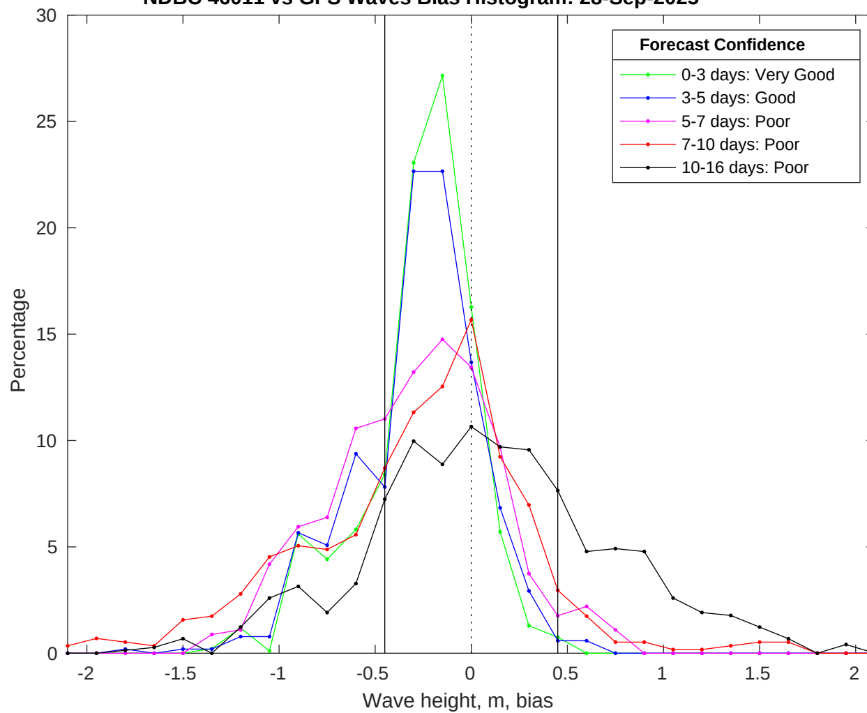
NDBC 46011 vs GFS Waves Bias Histogram: 28-Sep-2025
