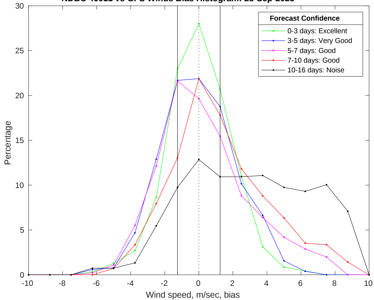
NDBC 46011 vs GFS Winds Bias Histogram: 28-Sep-2025
