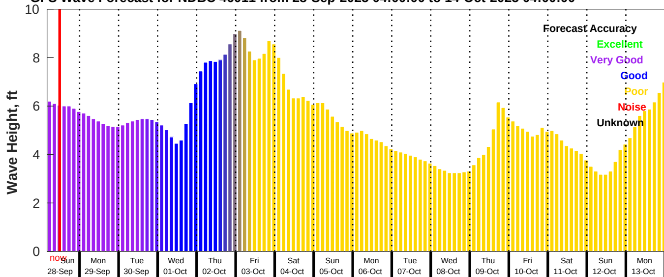
GFS Wave Forecast for NDBC 46011 from 28-Sep-2025 04:00:00 to 14-Oct-2025 04:00:00
