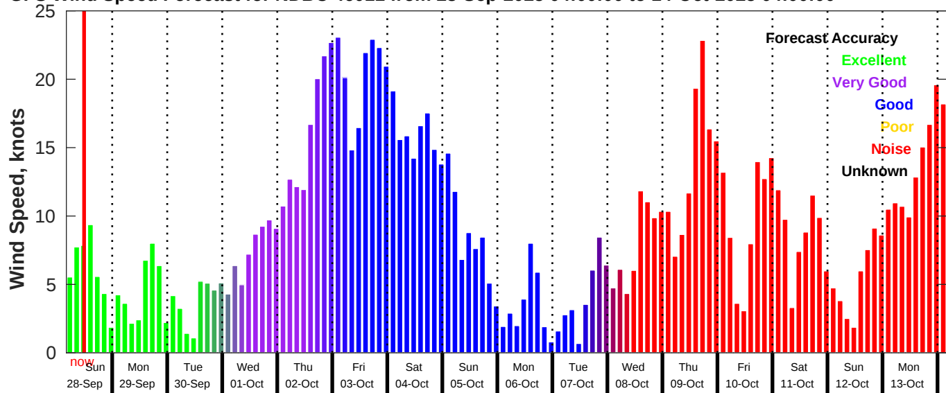
GFS Wind Speed Forecast for NDBC 46011 from 28-Sep-2025 04:00:00 to 14-Oct-2025 04:00:00
